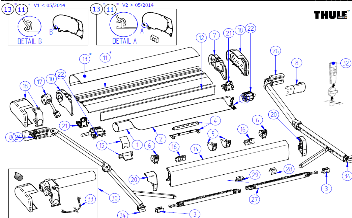
THULE Omnistor 9200
