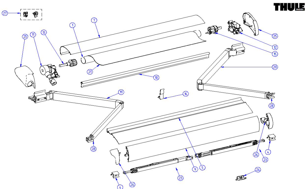
THULE Omnistor 6002
