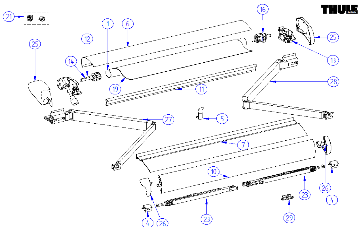
THULE Omnistor 6900
