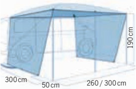
Light gray version with diagonally braced side panels
